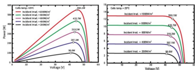
IV Curve Variation with irradiance
